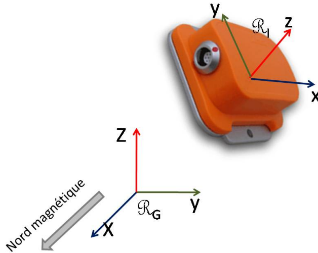
FIGURE 4.9: Centrale Inertielle
